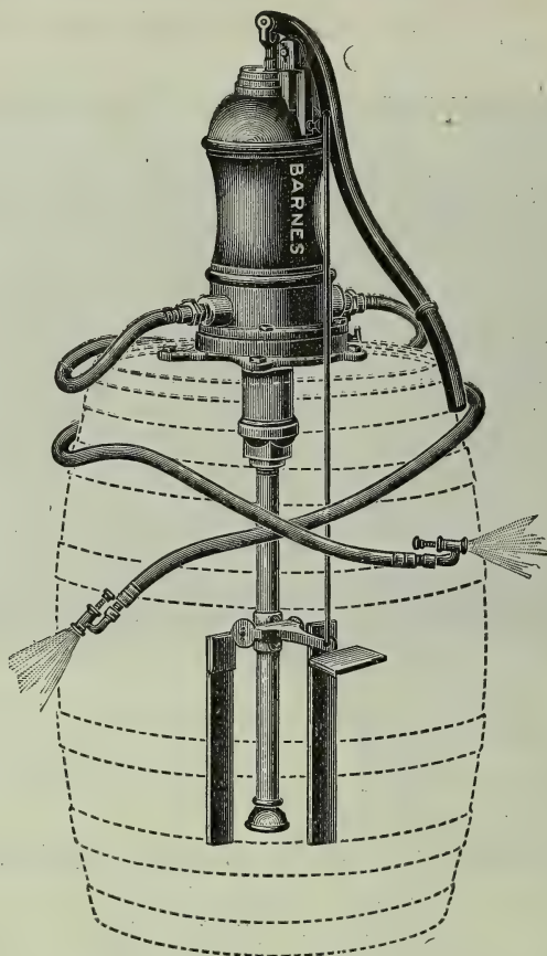
Barnes' New Improved Barrel Spray Pump
